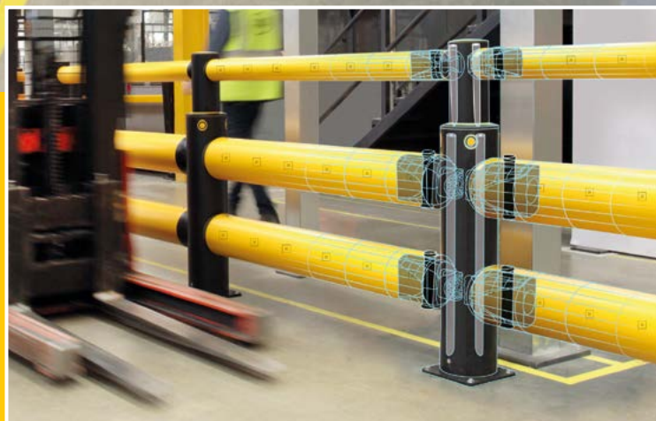
iFlex Double Traffic Barrier
