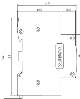
1, 2-contact versions
