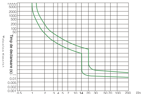
Caracteristica K
