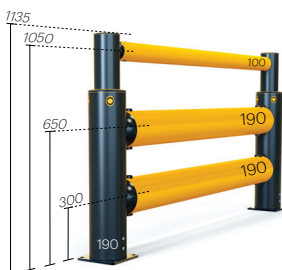
iFlex Double Traffic Barrier+ **
