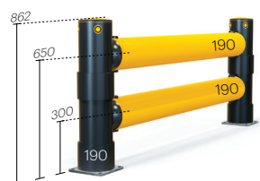
Atlas Double Traffic Barrier **
