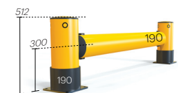
iFlex Single Rackend Barrier **
