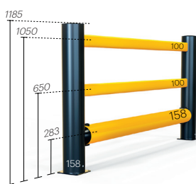
eFlex Single Traffic Barrier+ **
