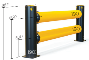
iFlex Double Traffic Barrier **
