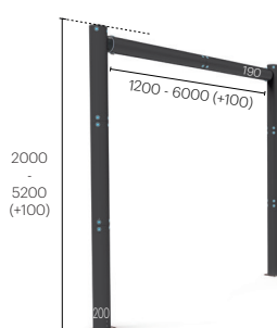
iFlex Cold Storage Height Restrictor ***
