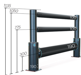
iFlex Cold Storage Single Traffic Barrier+ **
