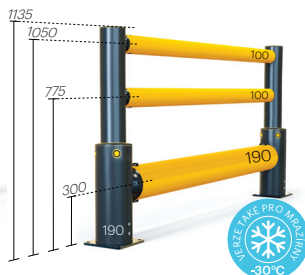
iFlex Single Traffic Barrier+ **
