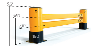
eFlex Double Rackend Barrier **
