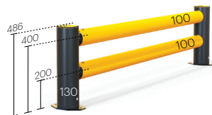
mFlex Double Traffic Barrier *
