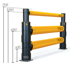
Atlas Double Traffic Barrier+ **
