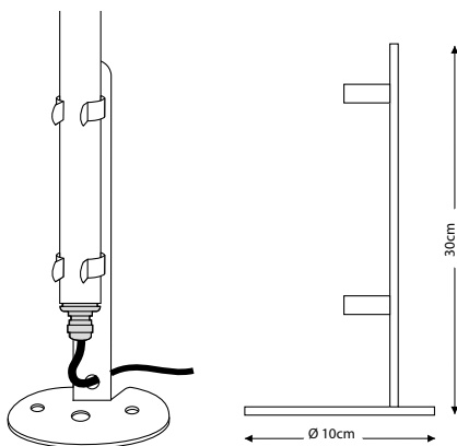
90106009 Picchetto INOX - Verticale Single INOX stake - vertical Einzeppflock INOX - vertikal
