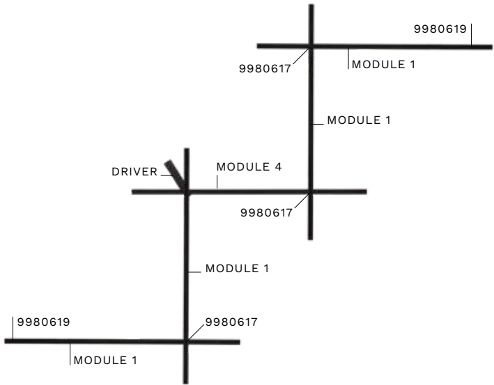
CONNECTIONS FOR 5 MODULES
