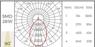
Light Distribution - High efficiency
