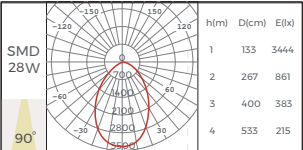
Light Distribution - Regular
