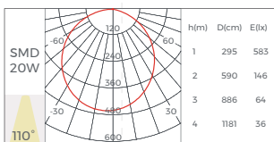
Light Distribution - White Light
