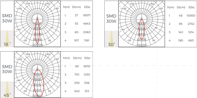
Light Distribution - White Light
