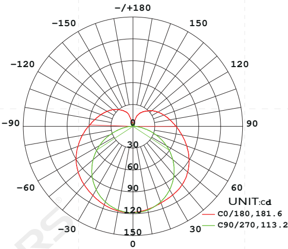
Light distribution
