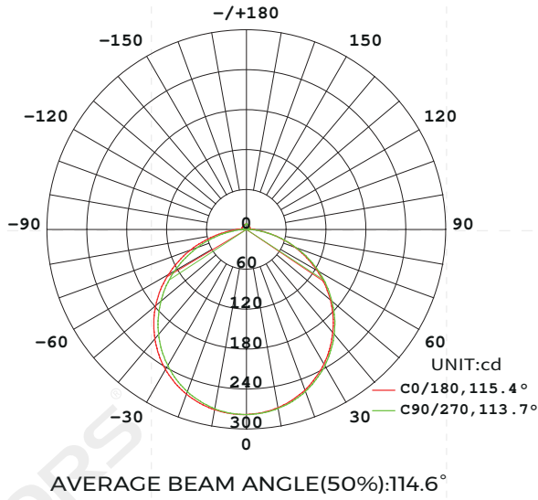
Light distribution
